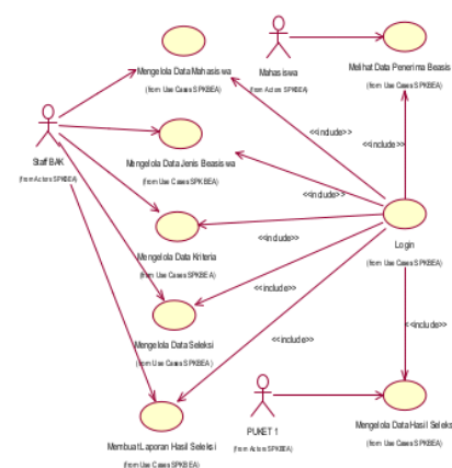
Gambar 3. Use Case Diagram SPK Beasiswa
