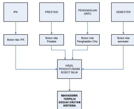
Gambar 2. Perhitungan Bobot Nilai
